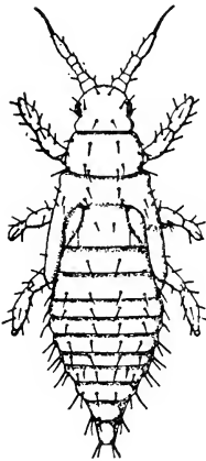
Fig. 67. Green house thrips, Heliothrips haemorrhoidalis (Bouche).
